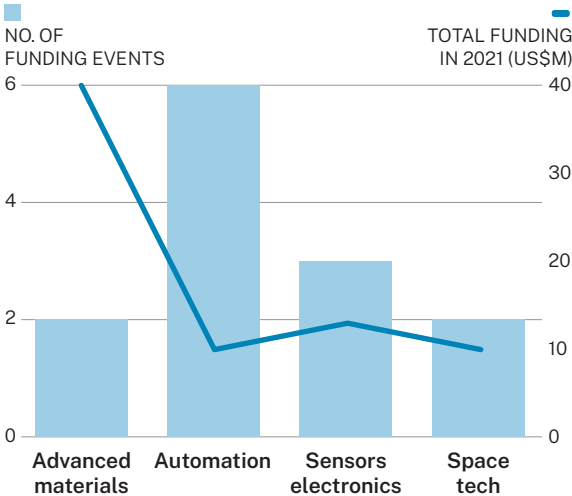
No. of funding events and total funding in 2021 (US$m)
